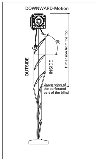
Models IF 50 ES / IF 80 ES Interior Venetian blind, freely suspended Operation: endless cord drive Slats: 50/80 mm
